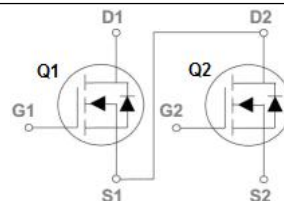
Schematic Diagram
