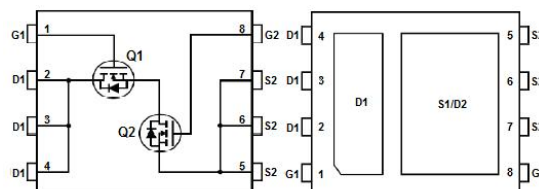
pin assignment
