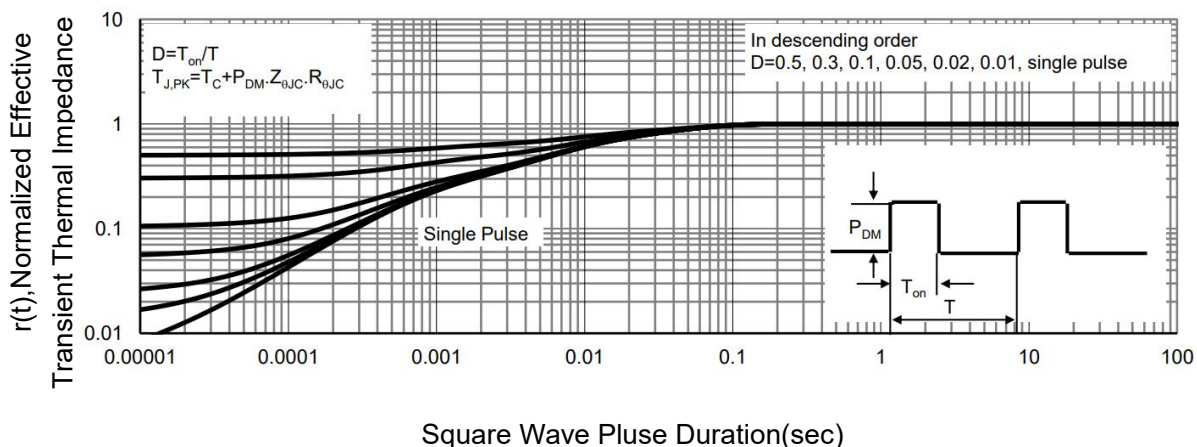
Square Wave Pluse Duration(sec) Figure 11 Maximum Transient Thermal Impedance
