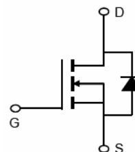
Schematic Diagram
