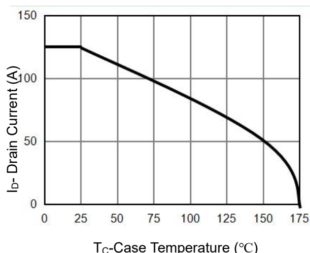
Figure 10 Current De-ratin
