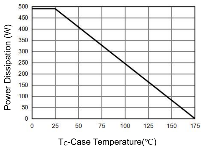
Figure 9 Power De-rating
