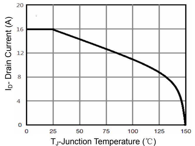
Figure 10 Current De-ratin
