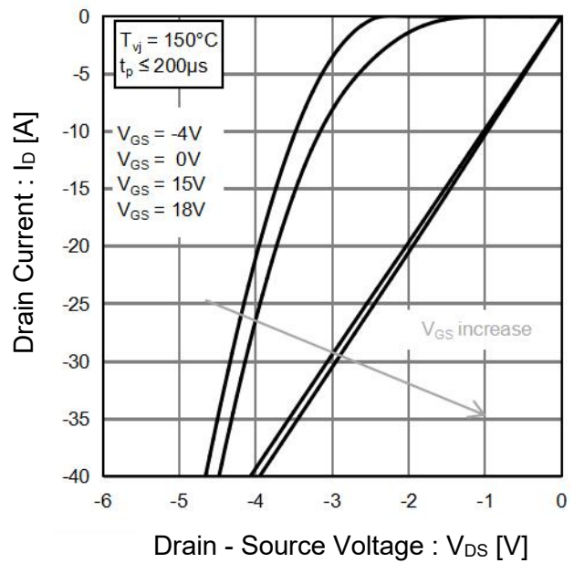
Fig.7 T_{vj} = 150^{\circ}C 3rd Quadrant Characteristics
