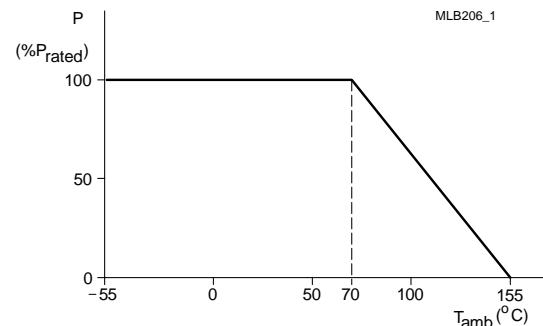
Fig. 3 Maximum dissipation ( P_{\max} ) in percentage of rated power as a function of the operating ambient temperature ( T_{\text{amb}} )
