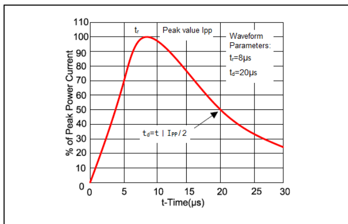
Figure 1. Pulse Waveforms
