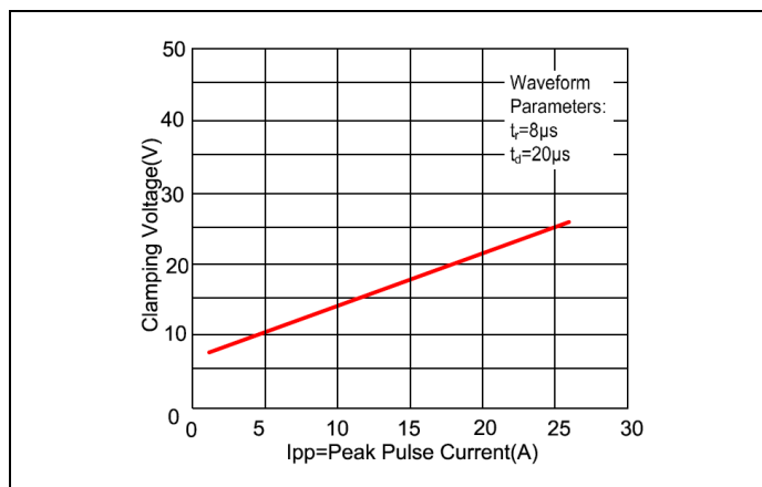
Figure 2. Clamping Voltage vs. Peak Pulse Current
