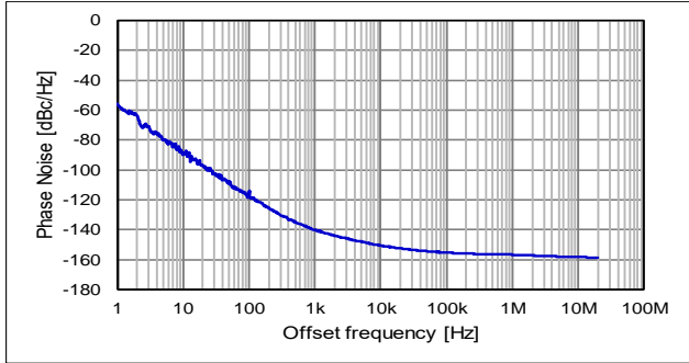
Phase Jitter (Offset frequency: 12 kHz to 20 MHz)
