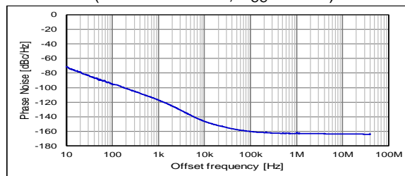
Phase Jitter (12 kHz to 20 MHz): 44 fs Typ.
