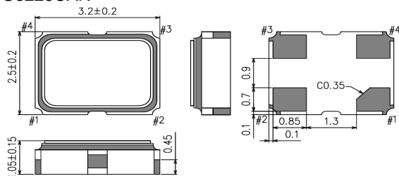
SG3225CAN
