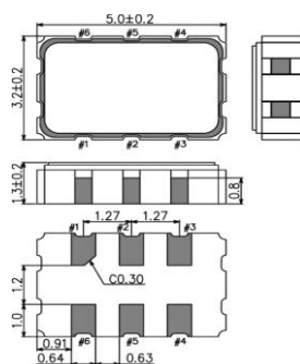
SG5032VEN
