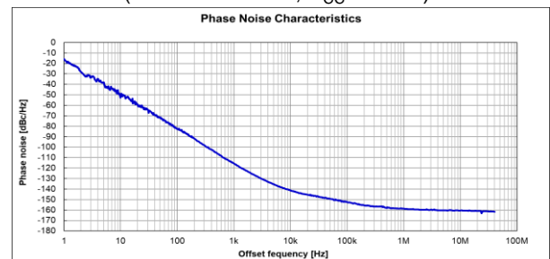
Phase Jitter (12 kHz to 20 MHz): 20 fs Typ.
