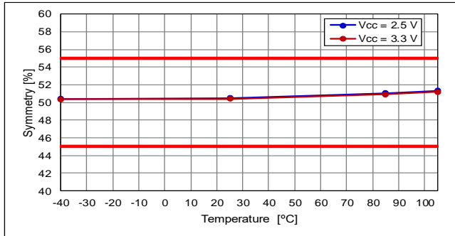
fo = 350 MHz
