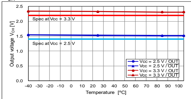
V OH
