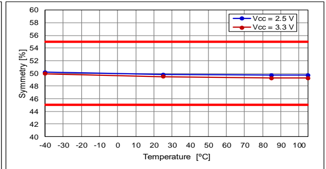
fo = 491.52 MHz
