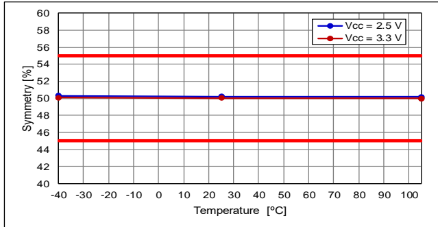
fo = 100 MHz
