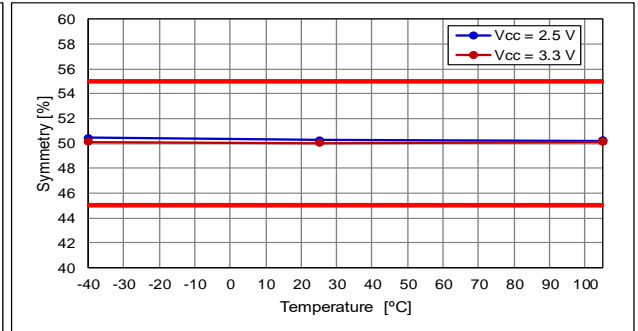
fo = 200 MHz
