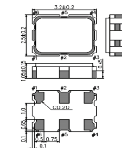
SG3225VEN
