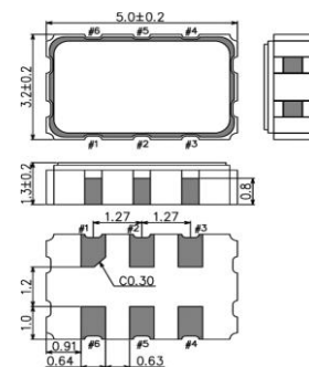
SG5032VEN
