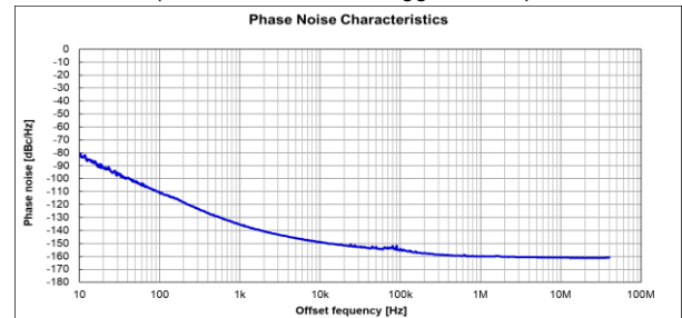
Phase Noise (fo = 156.25 MHz, V CC = 3.3 V)
