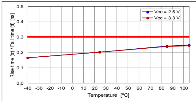
Rise Time
