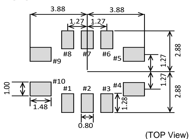
[ 9 ] Recommended Foot Print unit: mm
