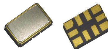
TG5032CKN TG5032SKN (10 pins)
