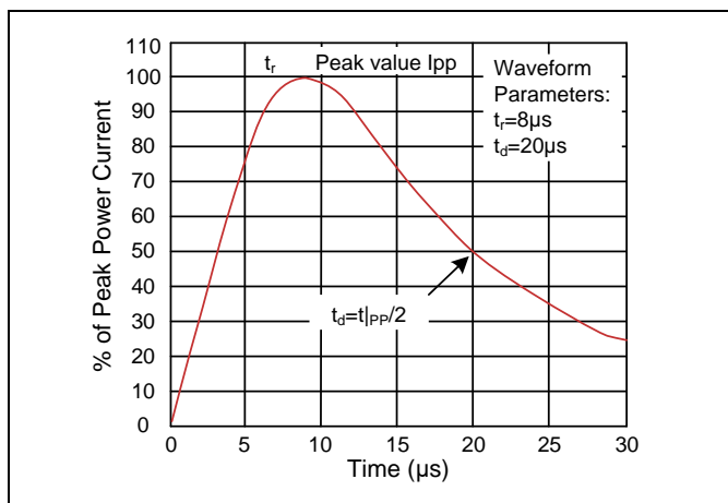
Figure 3. Pulse Waveform
