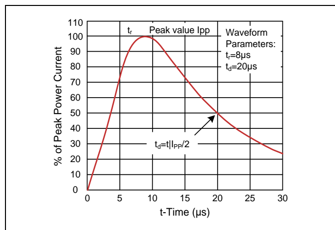
Figure 2. Pulse Waveforms
