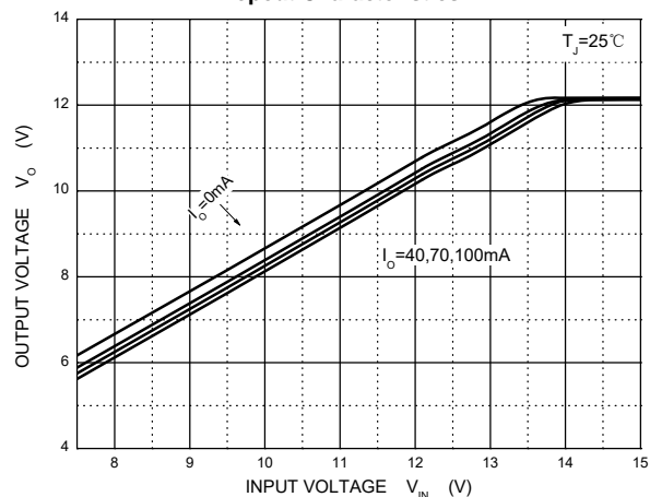
Dropout Characteristics
