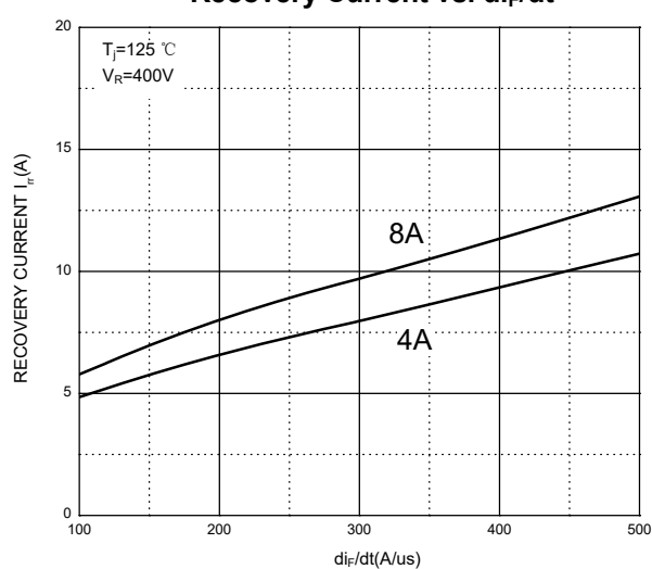
Recovery Current vs. di_F/dt
